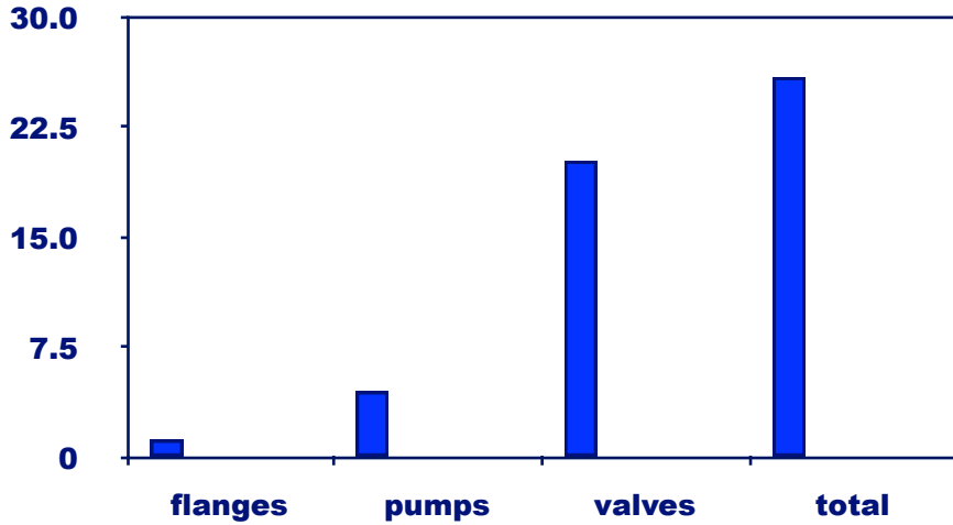
Figure 2 Baseline Plant Fugitive Emissions
