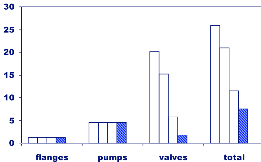
Figure 5 Possible Emission Levels With All Leaking Valves Repaired
