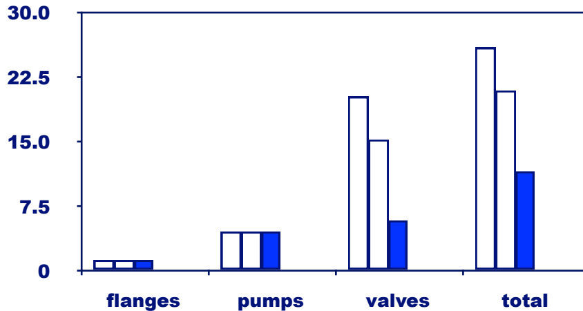
Figure 4 Plant Fugitive Emissions After Tightening Valve Glands
