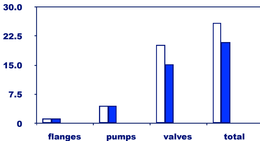
Figure 3 Plant Fugitive Emissions After Repacking Valves
