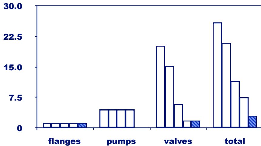
Figure 6 Possible Emission Levels With All Pump Seal Emissions Removed
