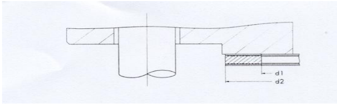
Camprofile Gaskets for ASME B16.5 Male / Female Flanges, Styles M20 and M40L, According to CAM 104 Standard (150 – 1500 Lbs)
